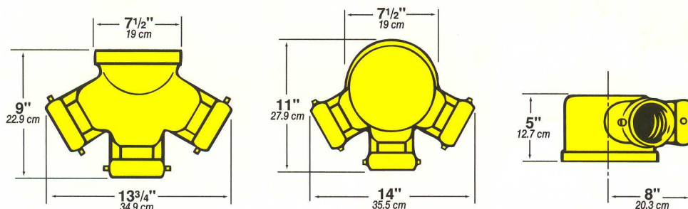
Angle Outlet
