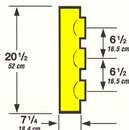
Model 5892 6" Female 15.2 cm NPT Both Ends
