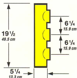
Model 5890 4" Female 10.2 cm NPT Both Ends
